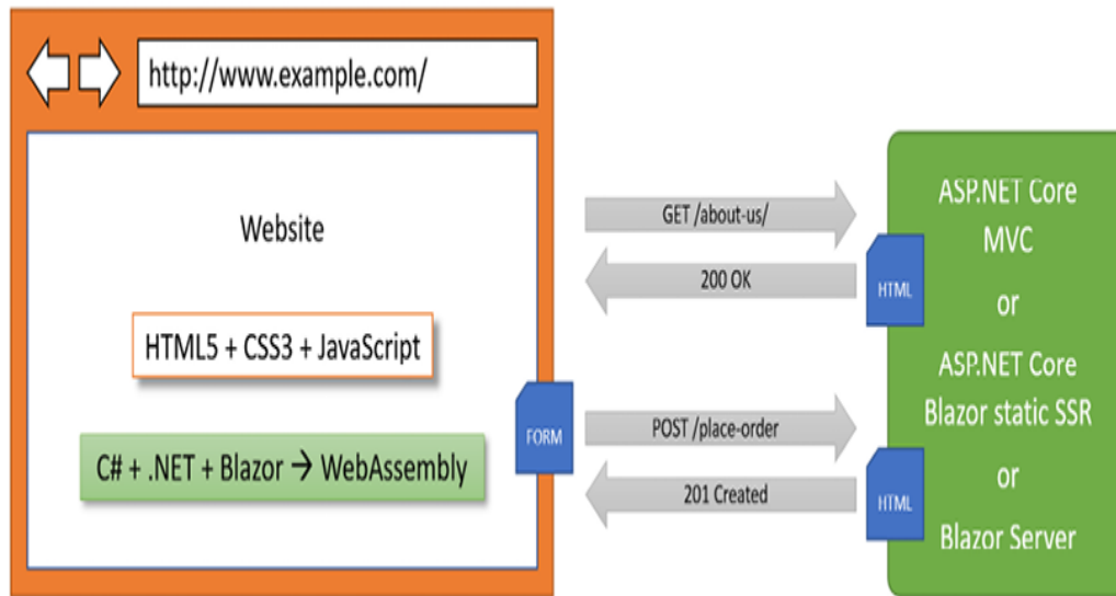
Figure 12.2: The use of C# and .NET to build websites on both the server side and client side
