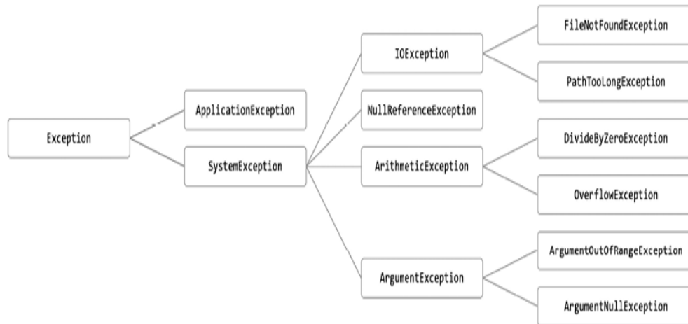
Figure 11.4: A partial exception inheritance hierarchy
