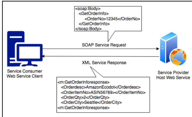
SOAP-based web service
