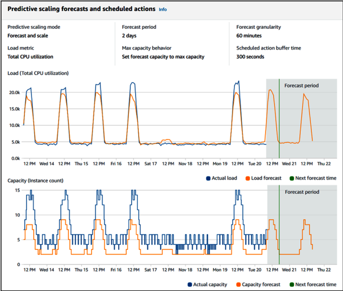
Predictive scaling forecast
