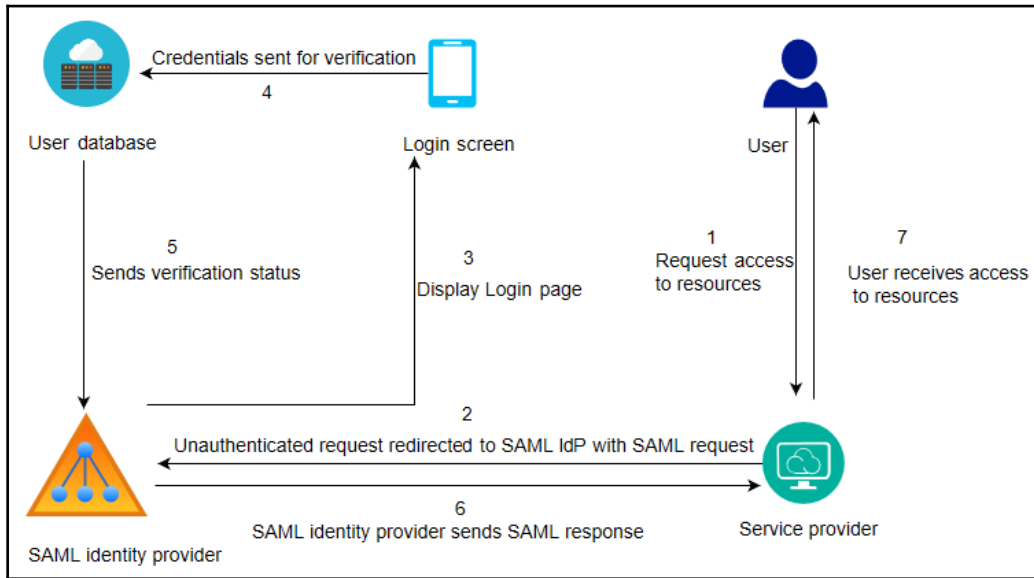
User authentication using SAML
