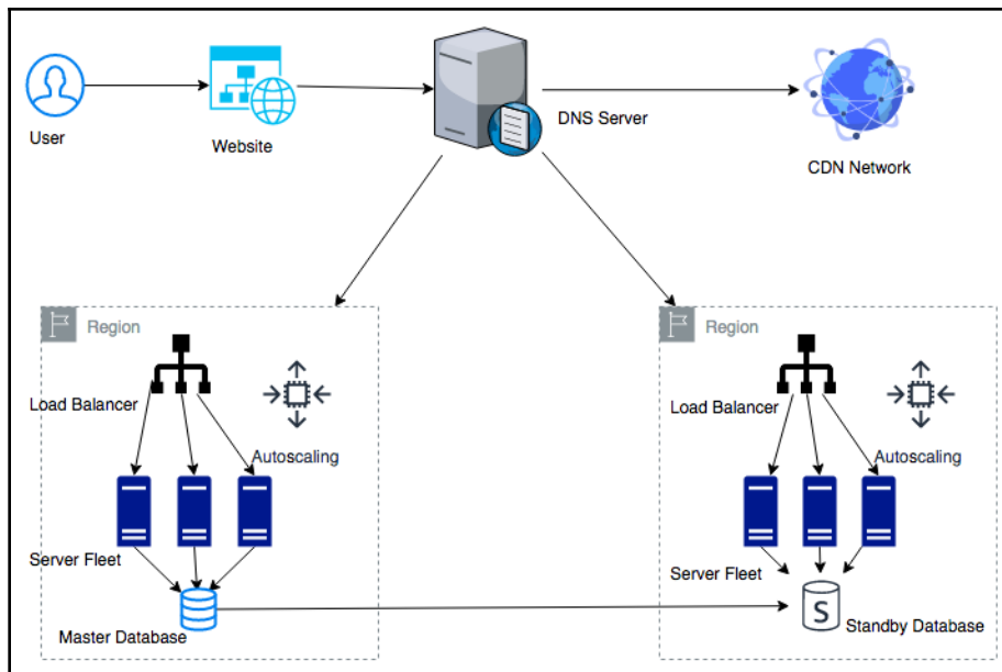
Application architecture resiliency
