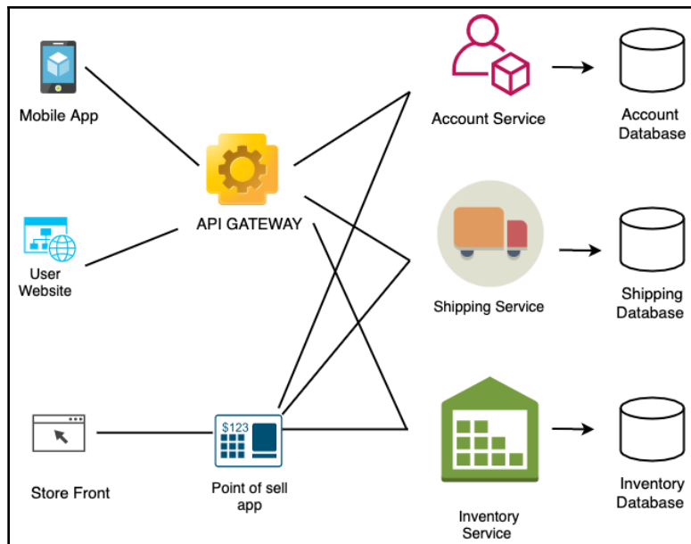
Conceptual architecture diagram of an e-commerce platform
