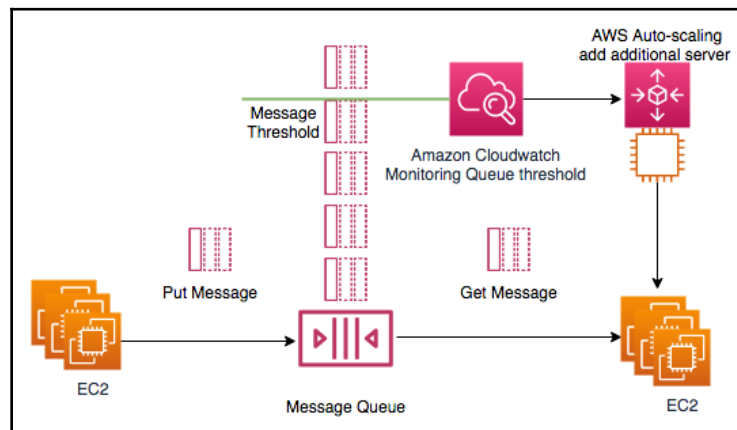
Job observer pattern architecture
