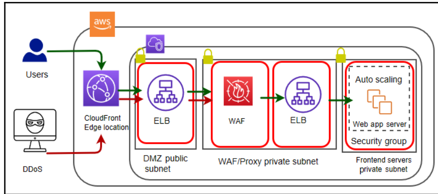
DDoS WAF sandwich mitigation strategy
