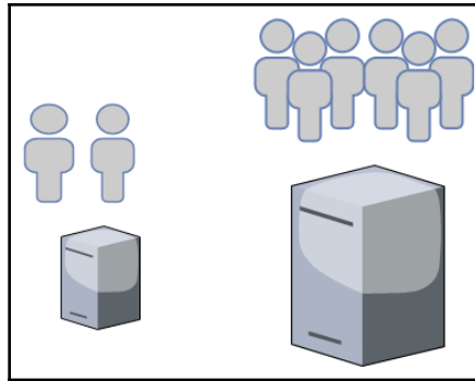
Vertical scaling
