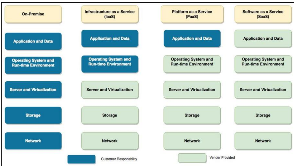
Type of cloud computing model
