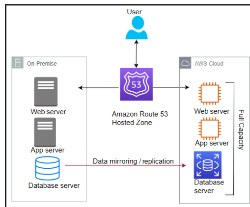
Multi-site scenario running an active-active workload with a full capacity
