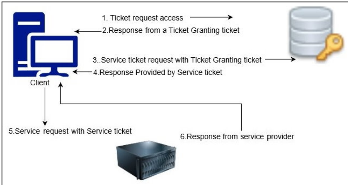
Kerberos authentication
