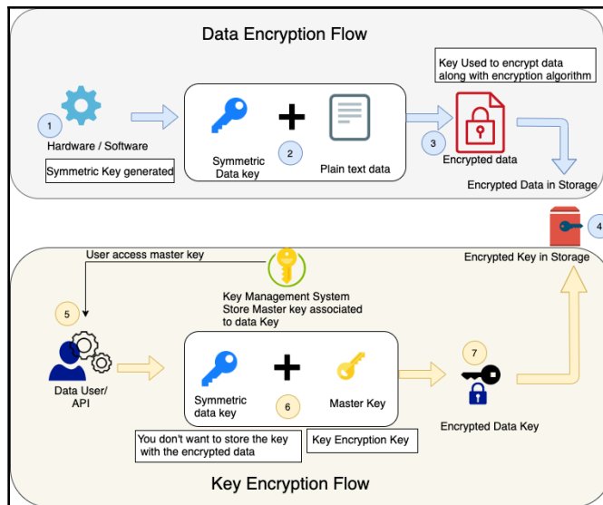
Envelope encryption
