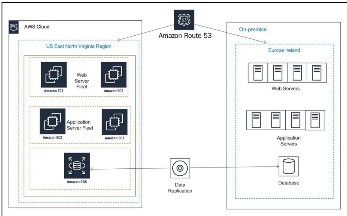
Hybrid multi-site disaster recovery architecture
