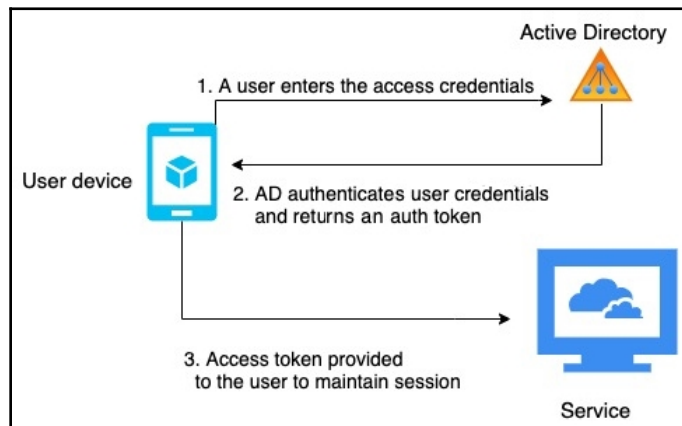
AD authentication flow
