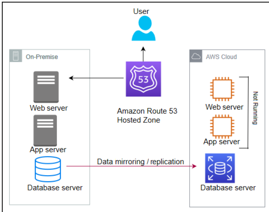
The pilot light data replication to DR site scenario
