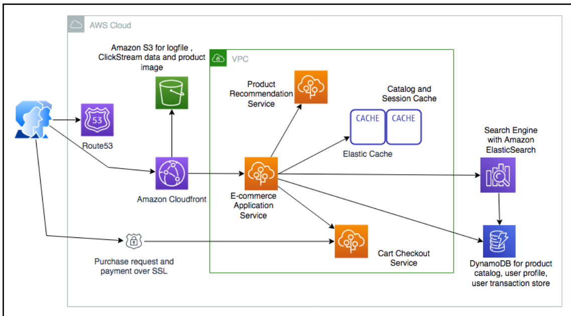
E-commerce website SOA architecture
