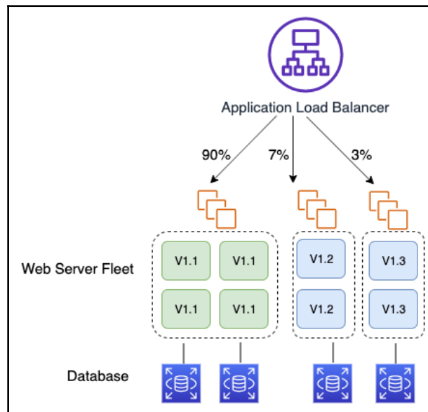
Split users by feature experiment using A/B testing
