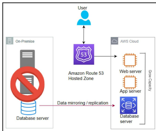
Recovery phase in the warm standby scenario
