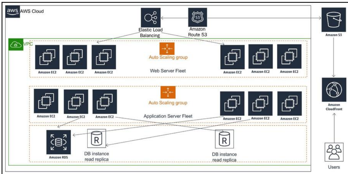
Scaling three-tier architecture
