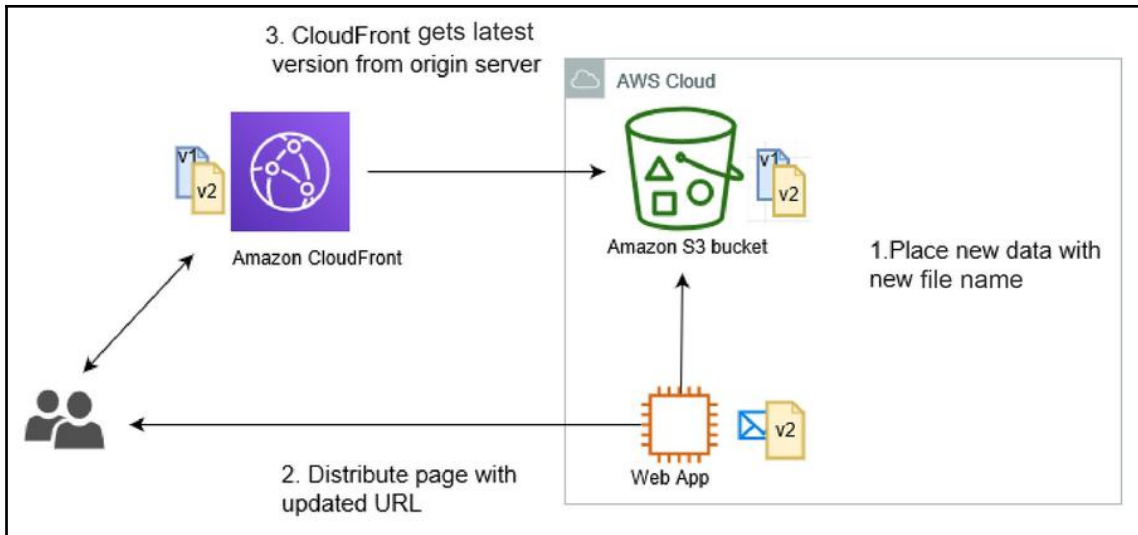
Rename distribution pattern architecture
