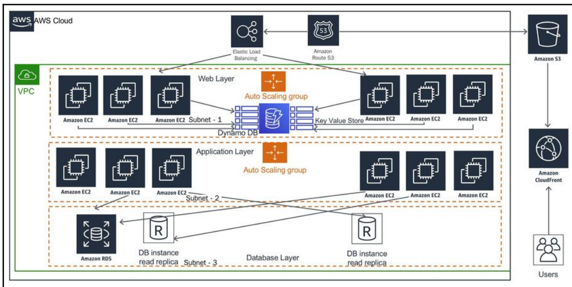
A stateless application architecture
