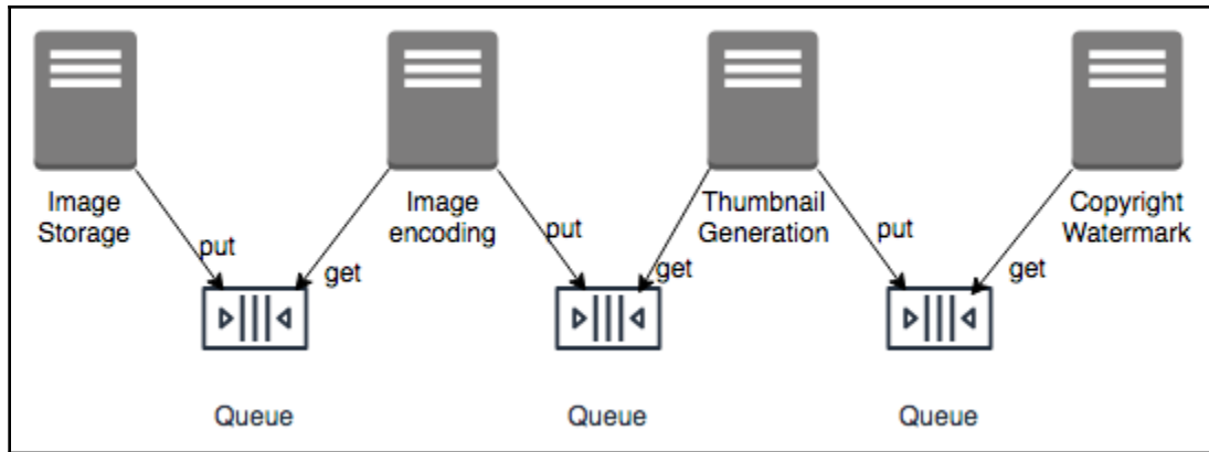
Queue-based loosely coupled architecture
