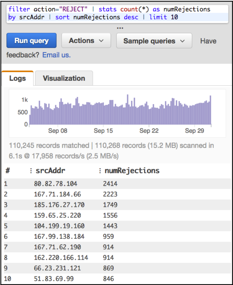
Insight from raw network log by running query
