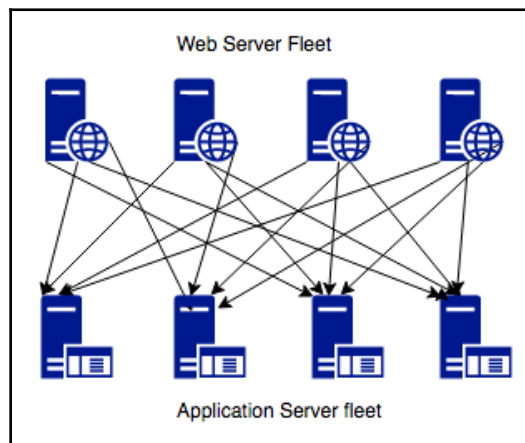
Tightly coupled architecture
