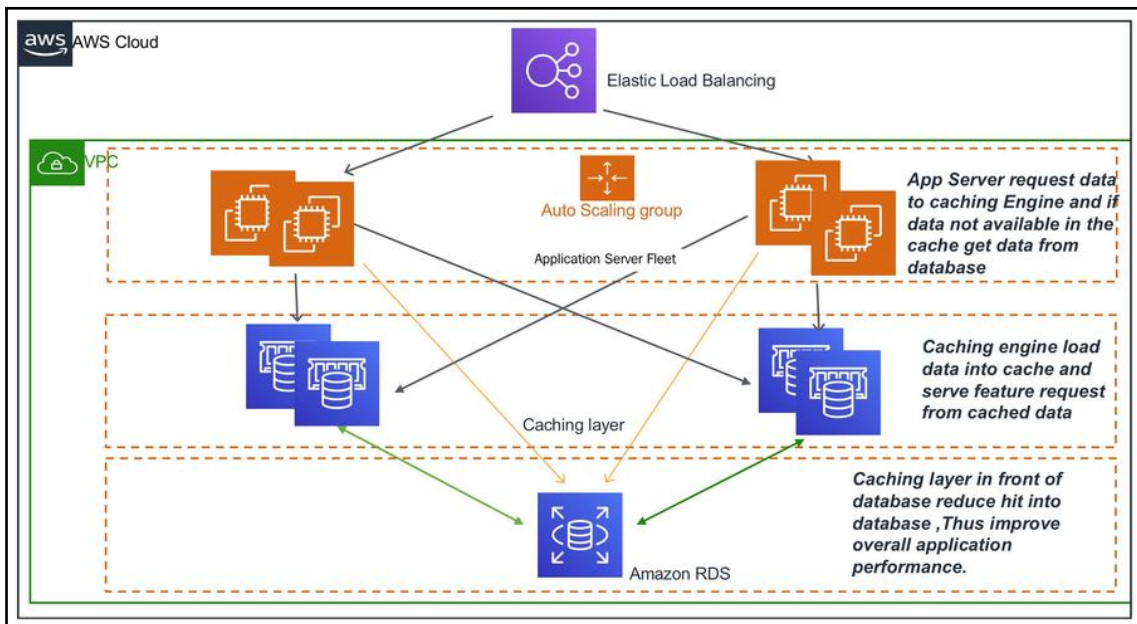
Application caching pattern architecture
