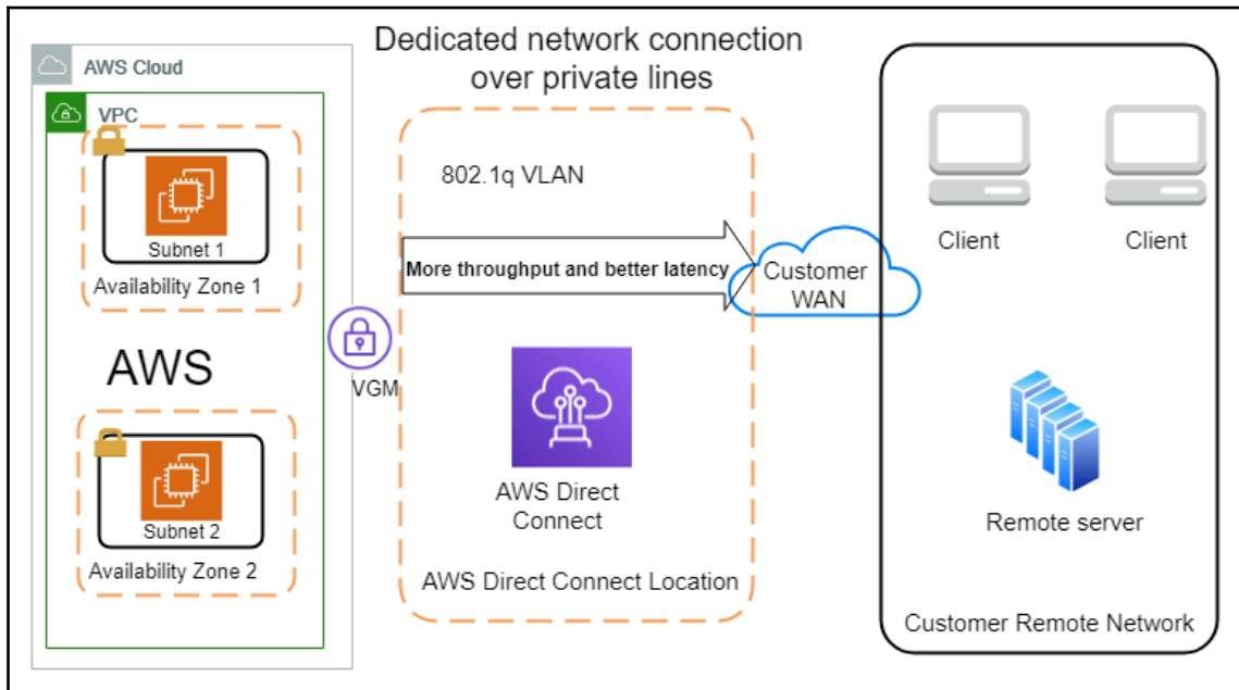
Hybrid cloud architecture (on-premise to cloud connectivity)
