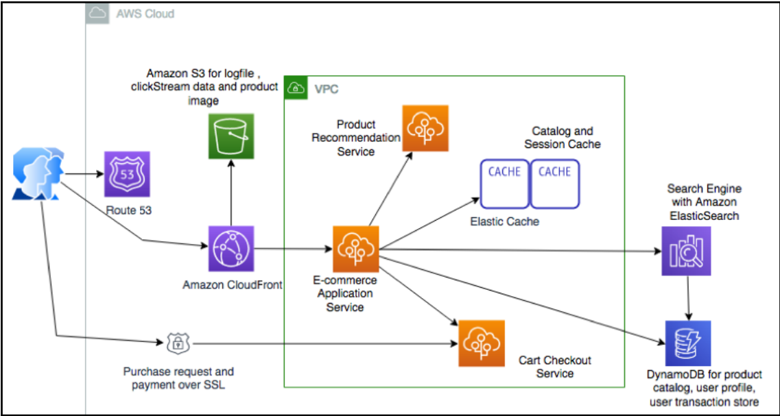
Application architecture diagram of an e-commerce platform
