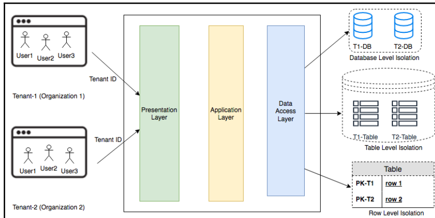
Multi-tenant SaaS architecture
