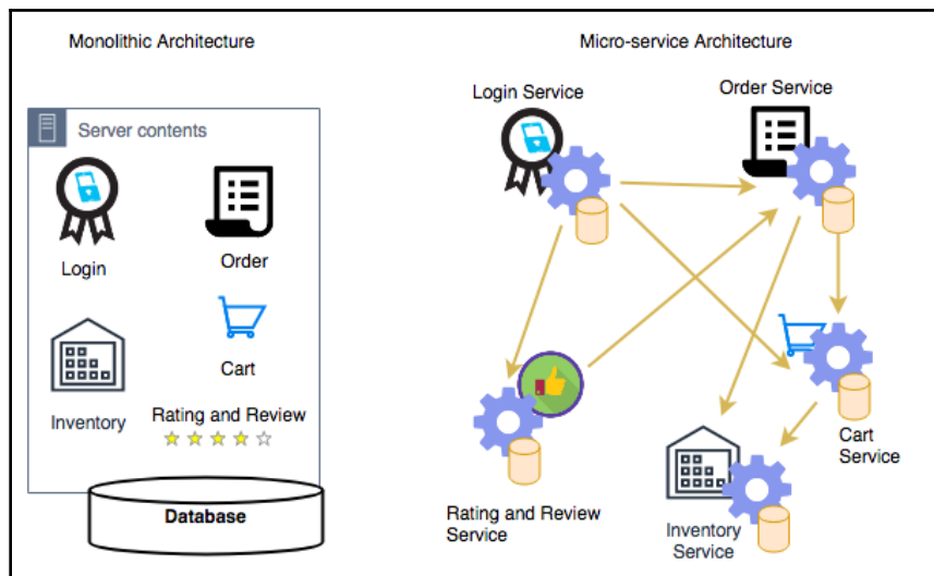
Monolithic to the microservice architecture
