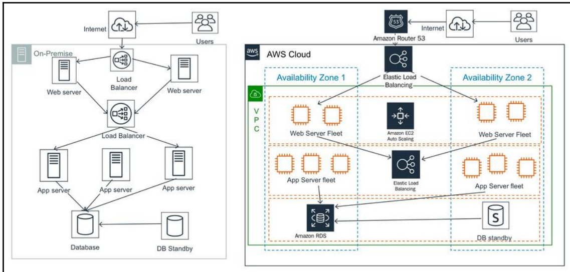
On-premise to AWS Cloud architecture
