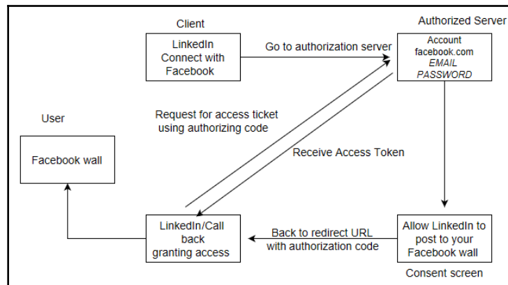
User access delegation with OAuth 2.0
