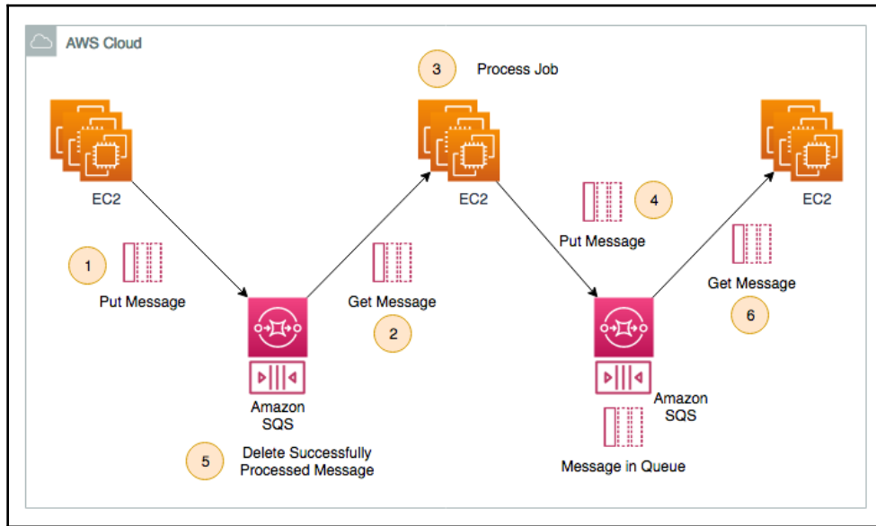
Queuing chain pattern architecture
