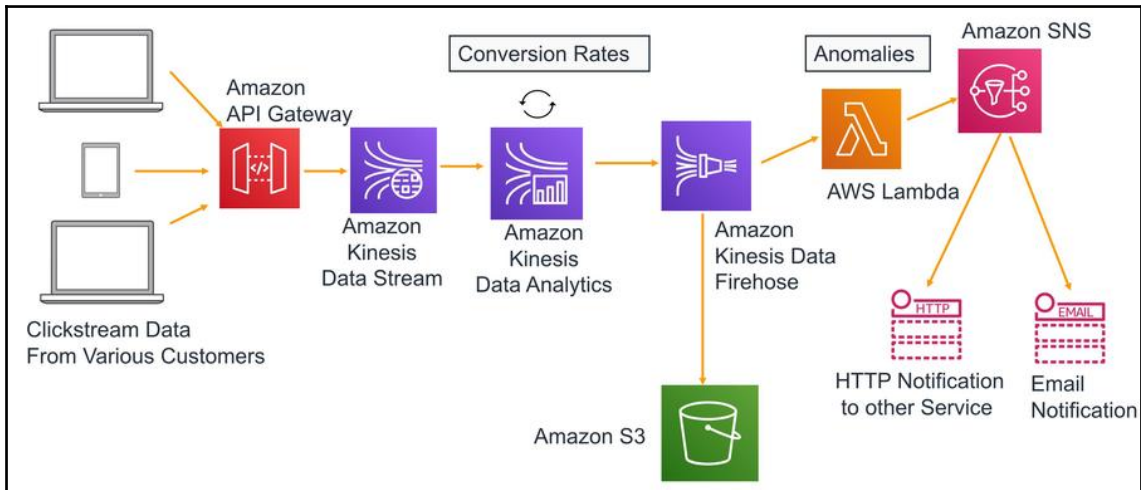
Clickstream analysis event stream architecture
