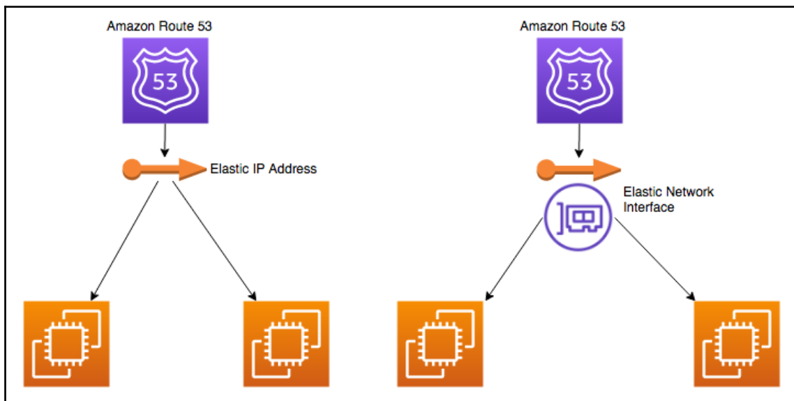
Floating IP and interface pattern
