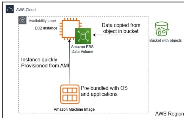
Restoring systems from Amazon S3 backups in the cloud
