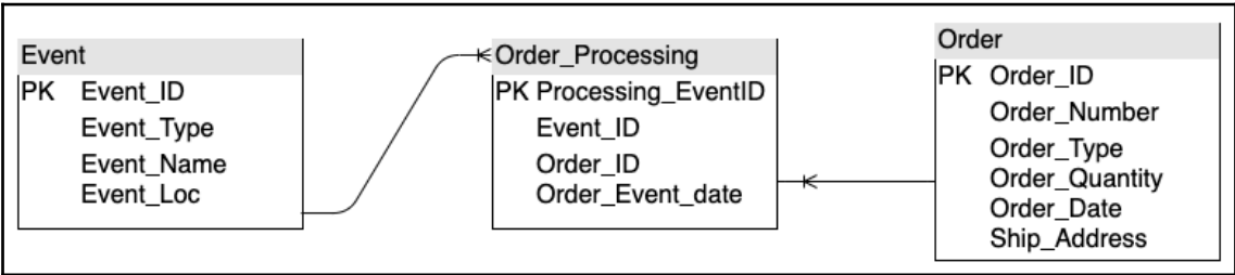
ER diagram of an e-commerce platform
