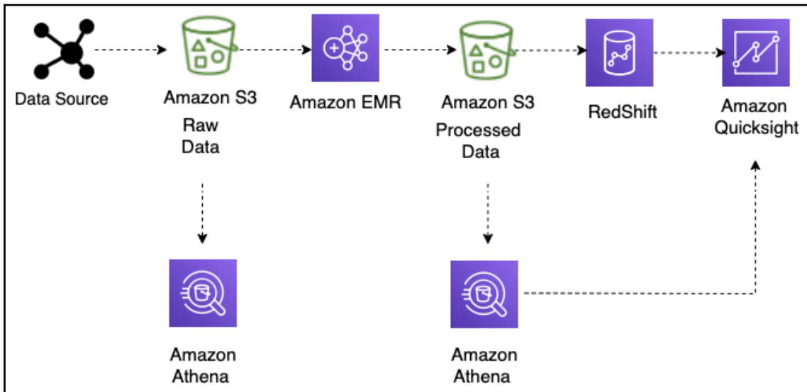
Data lake ETL pipeline for big data processing
