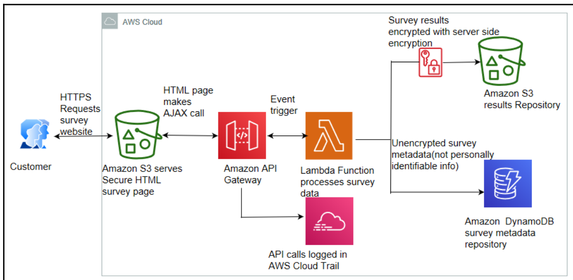
Serverless architecture for a secure survey delivery
