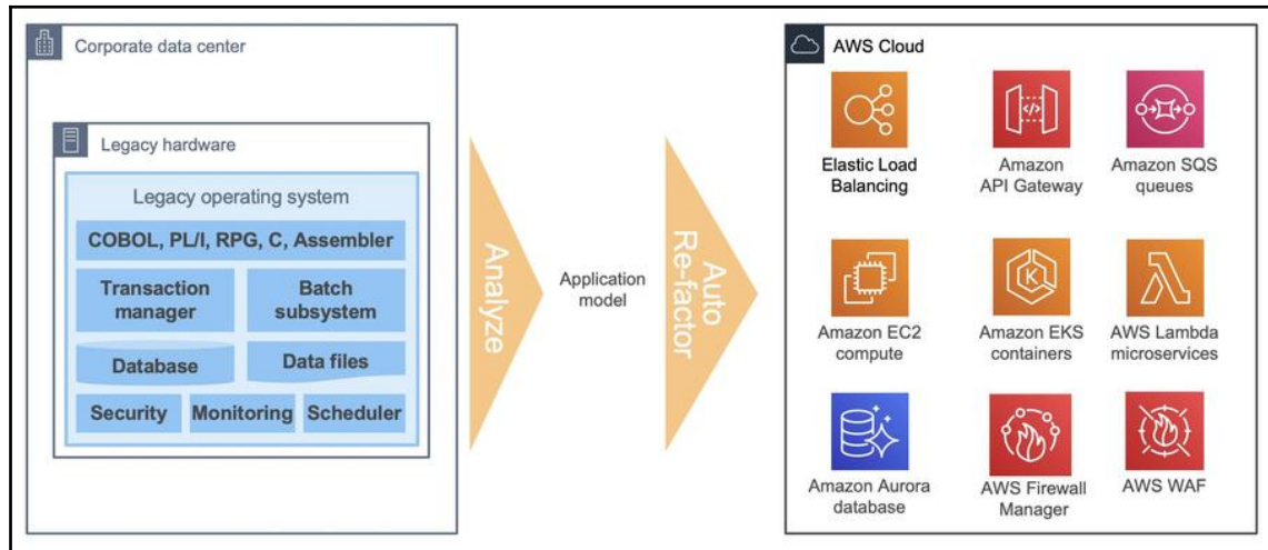
Legacy mainframe system modernization to the cloud
