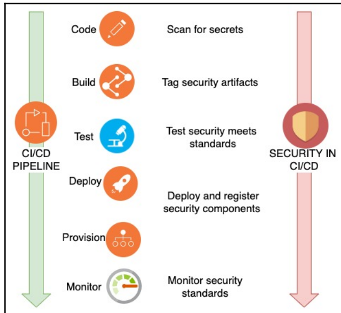
DevSecOps and CI/CD
