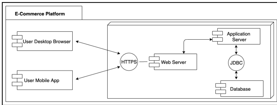
Deployment diagram of an e-commerce platform
