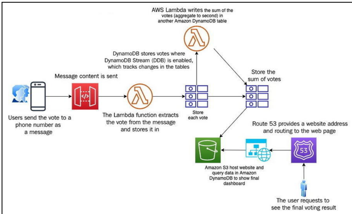
Microservice based real-time voting application architecture
