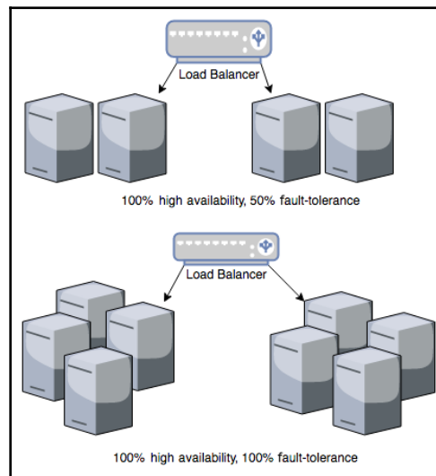
Fault-tolerance architecture
