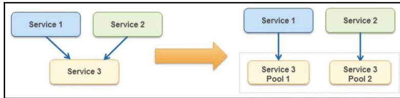
Bulkhead pattern
