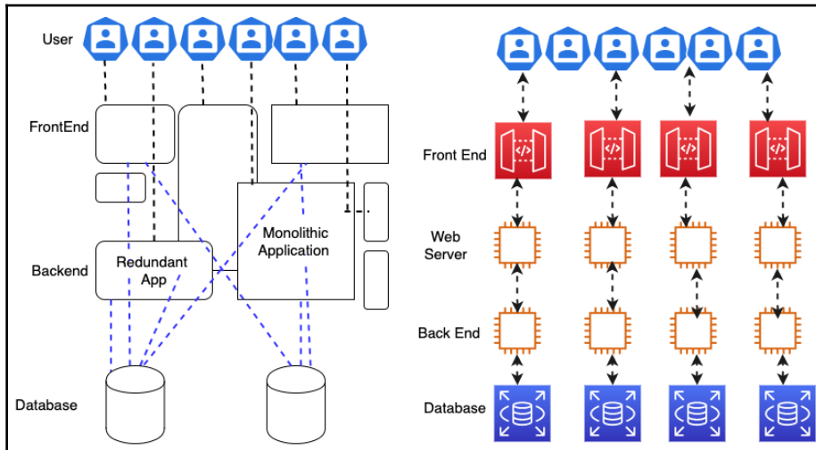
Architectural standardization
