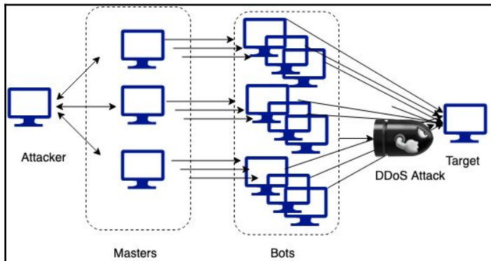
DDoS attack
