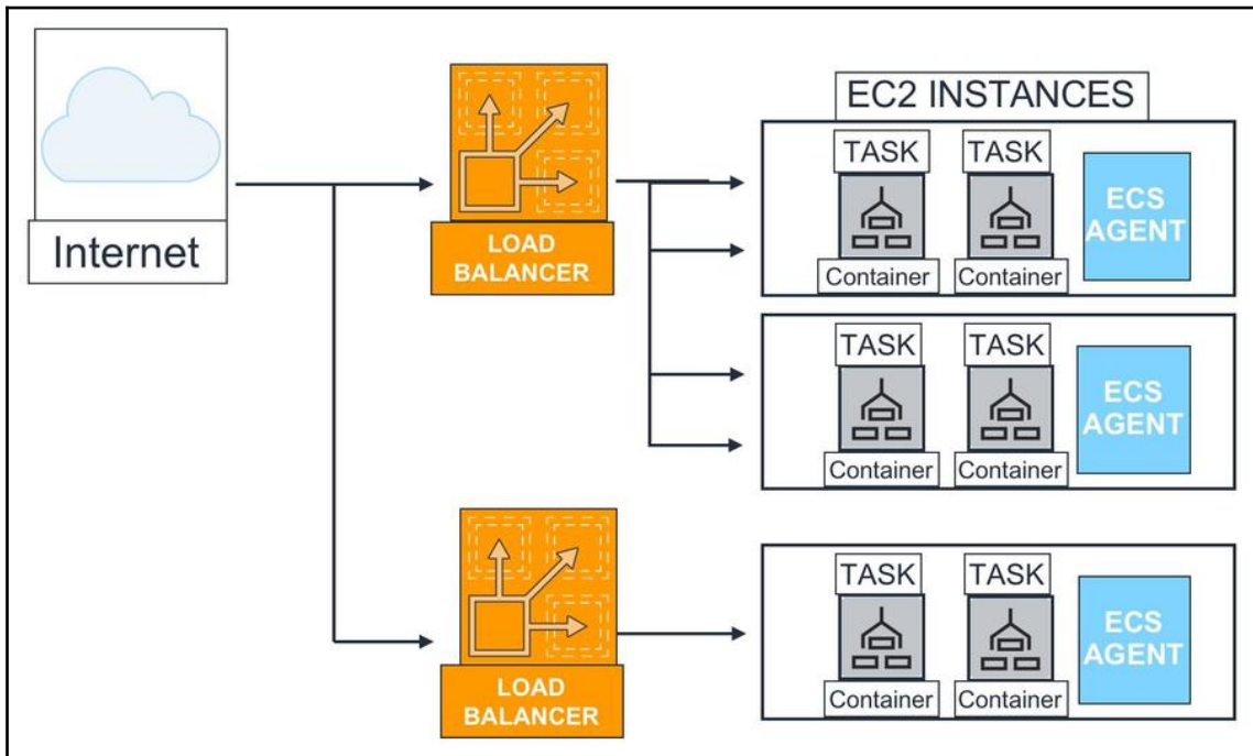
Container deployment architecture
