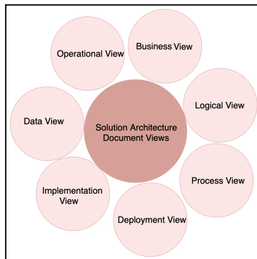
SAD views
