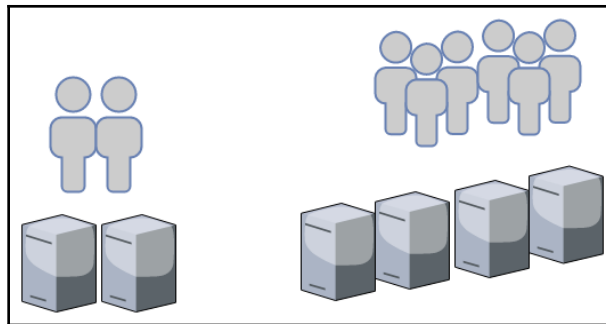
Horizontal scaling
