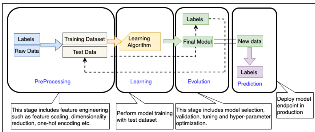
ML workflow
