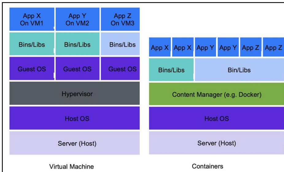
Virtual machines and containers for application deployment
