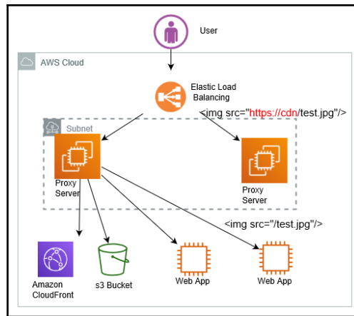
Rewrite proxy pattern architecture
