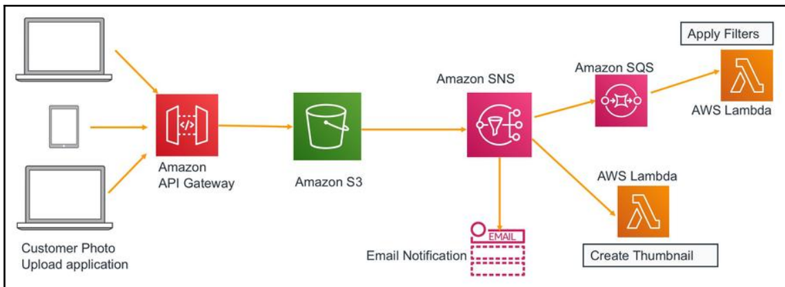
Photo studio application pub/sub-event-driven architecture
