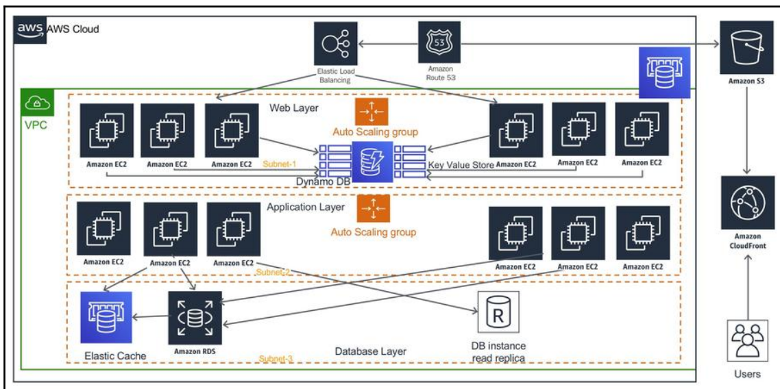
Cache distribution pattern architecture
