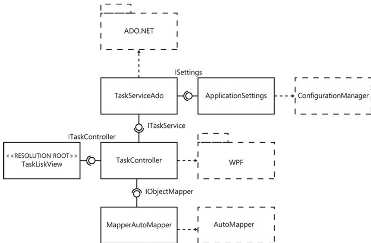
FIGURE 9-3 The interfaces, their implementations, and their dependencies, all of which make up the Task List application.
