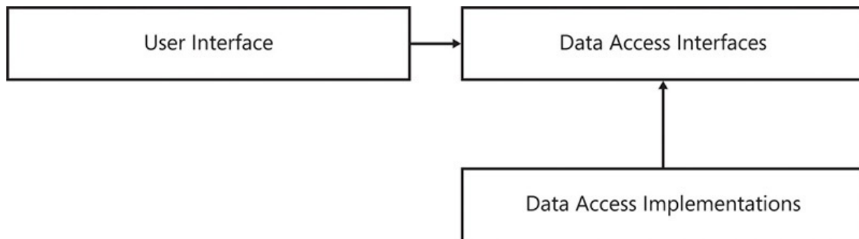
FIGURE 2-22 The two layers are separated into implementation assemblies and interface assemblies.
