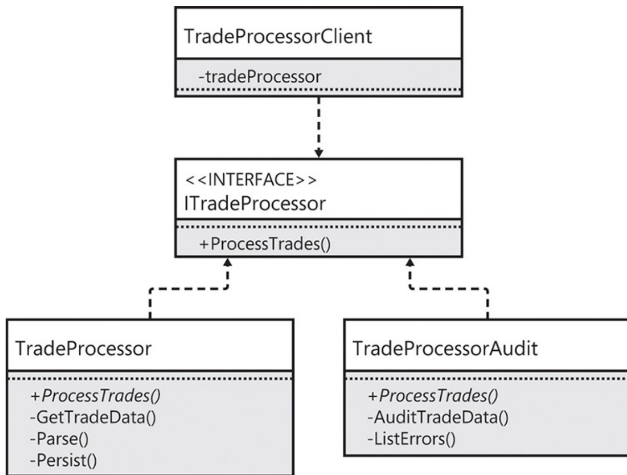
FIGURE 6-4 The client depends on an interface rather than a class.
