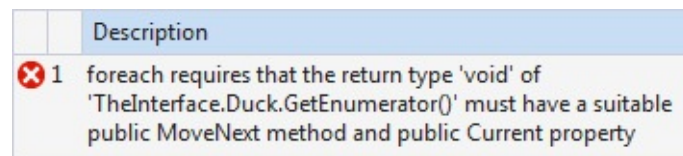
FIGURE 3-9 The return type of the GetEnumerator method must also match an implicit contract.
