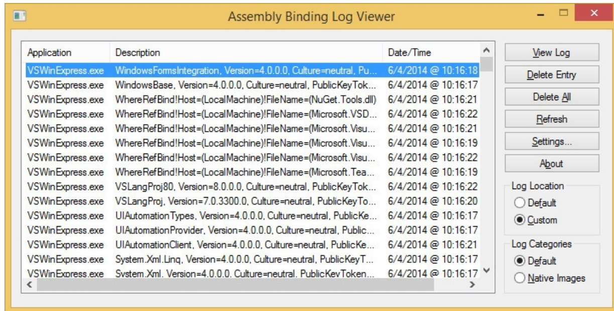
FIGURE 2-16 Fusion has a user interface for finding the log file for your application.
