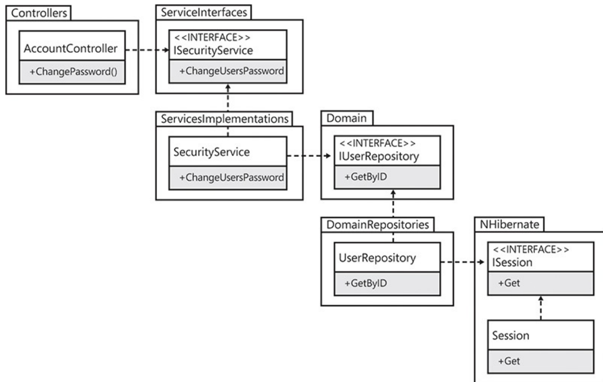
FIGURE 2-14 The Stairway pattern is aptly named.
