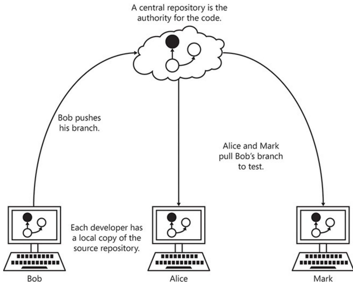
FIGURE A-2 Distributed source control is a peer-to-peer system, but it often uses a central repository.
