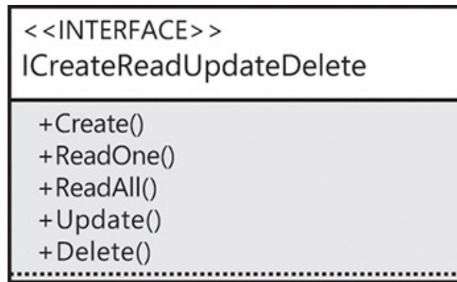
FIGURE 8-1 The initial interface before segregation.
