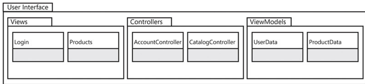
FIGURE 2-20 By grouping related assemblies together, you can define logical components.
