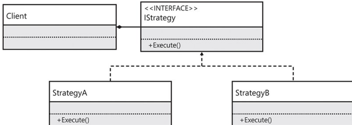
FIGURE 3-7 The UML class diagram of the Strategy pattern.
