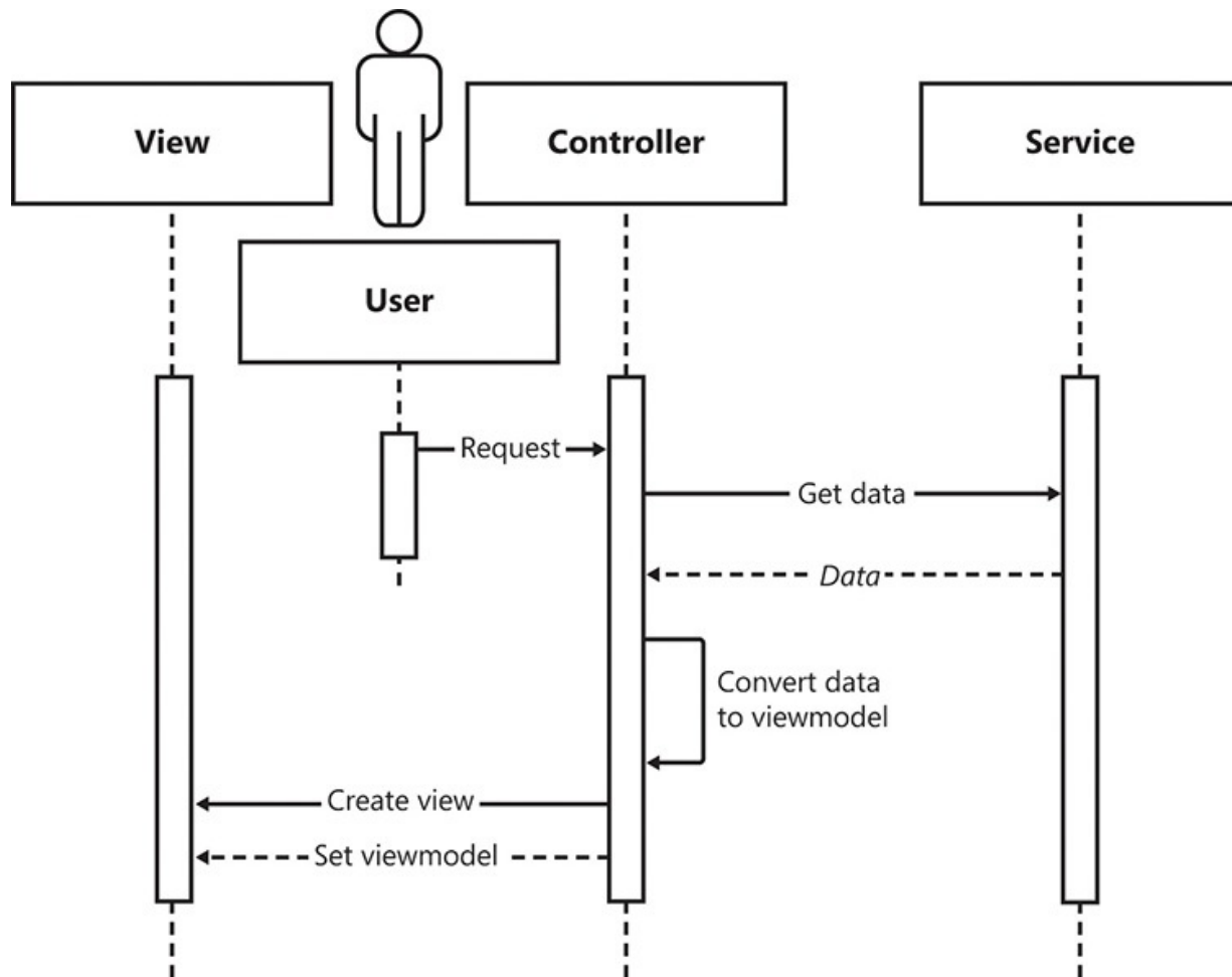
FIGURE 11-1 Dianne's sequence diagram generalizes the structure of the application.
