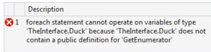
FIGURE 3-8 Without requiring a specific interface, the compiler complains that a public method is missing from the class.
