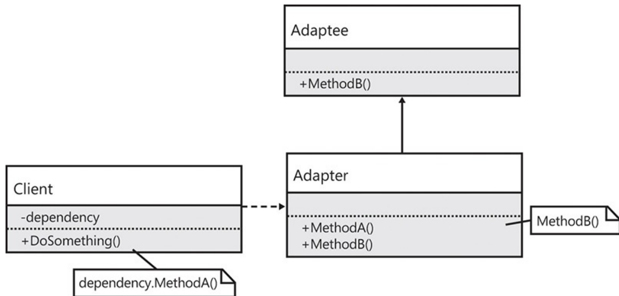
FIGURE 3-5 The UML class diagram for the Class Adapter pattern.
