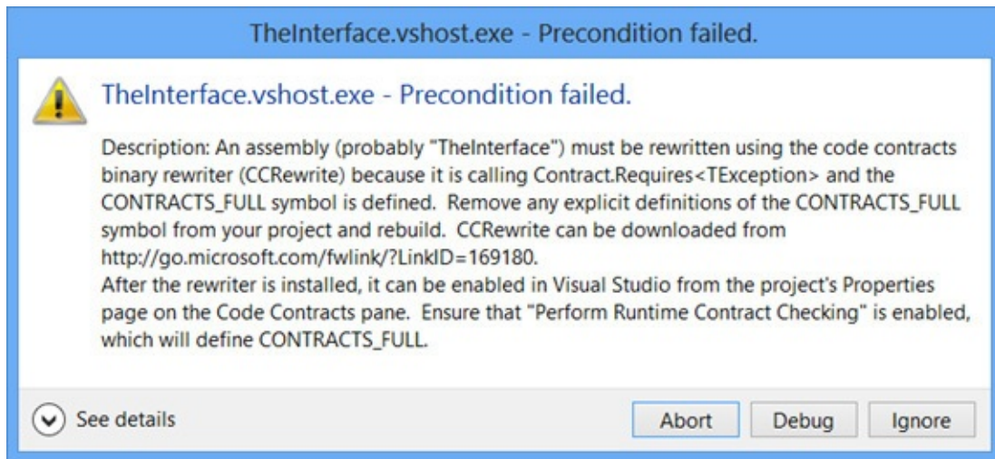
FIGURE 7-2 Code contracts must be configured before use.
